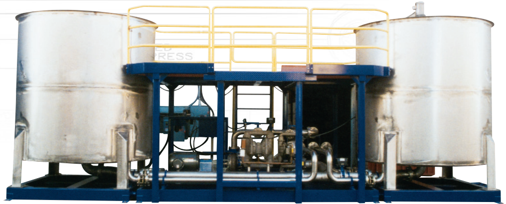
FTS40L3-S1, 100 cu.ft., support skid with (2) 3,000 gallon tanks.
